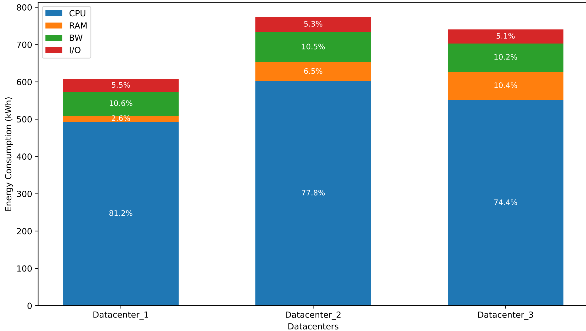
Baseline Scenario: Power Consumption per Datacenter (Stacked by Component)
